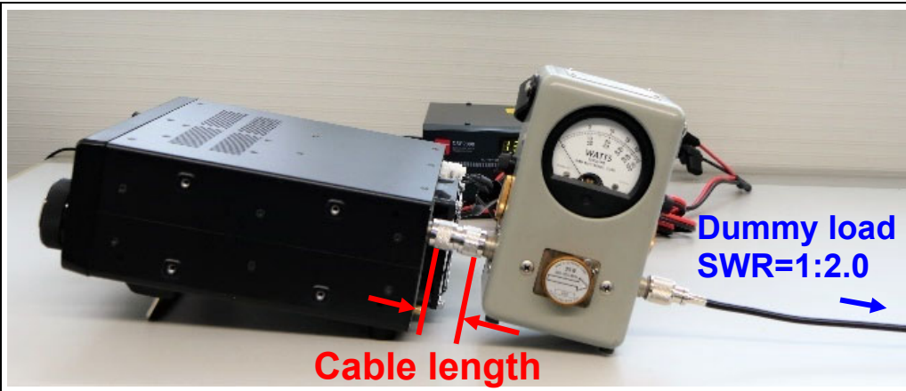
RF power is set at 10 W with a SWR=1:2.0 dummy load.
